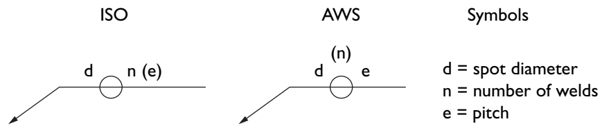
12.1 Symbolisation of a resistance spot weld.
