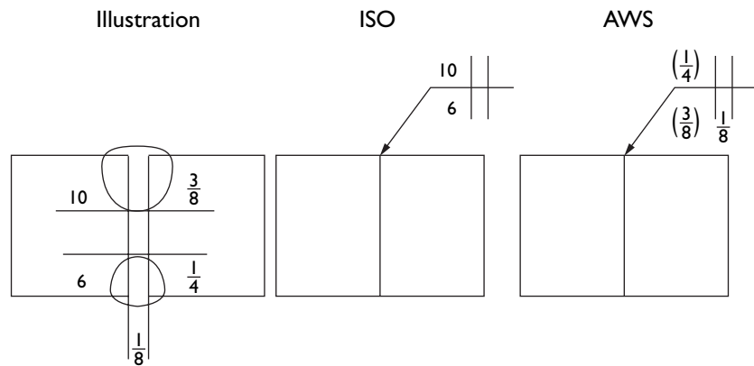
9.4 Partial penetration square butt/groove weld. ISO dimensions are in millimetres; AWS dimensions are in inches.
